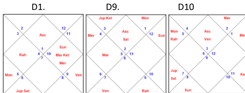
Planet Position Calculation
